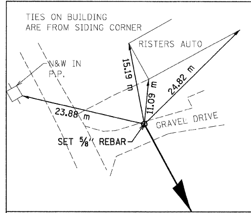
ELIZABETH STREET POT STA 0+066.707 N 255,693.3690 E 698,204.8960
