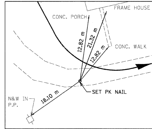
ELIZABETH STREET PI STA 0+097.709 N 255,666.0163 E 698,219.4874
