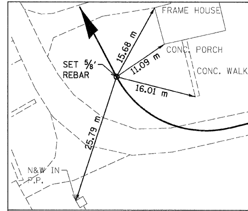
ELIZABETH STREET PC STA 0+082.153 N 255,679.7411 E 698,212.1658
