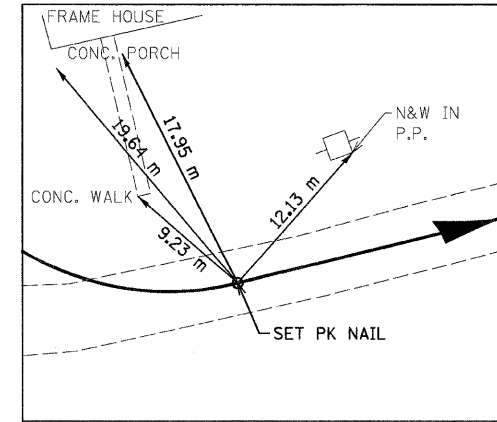
ELIZABETH STREET PT STA 0+108.595 N 255,669.7341 E 698,234.5921
