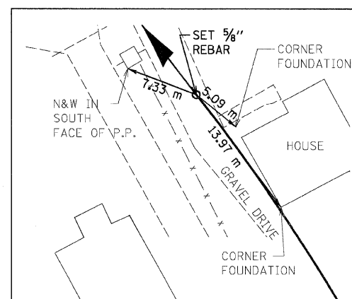
SERVICE DRIVE 1 PT STA 0+981.547 N 255,797.6232 E 698,316.0226
