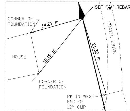
SERVICE DRIVE 1 PC STA 0+901.123 N 255,725.8487 E 698,350.9581
