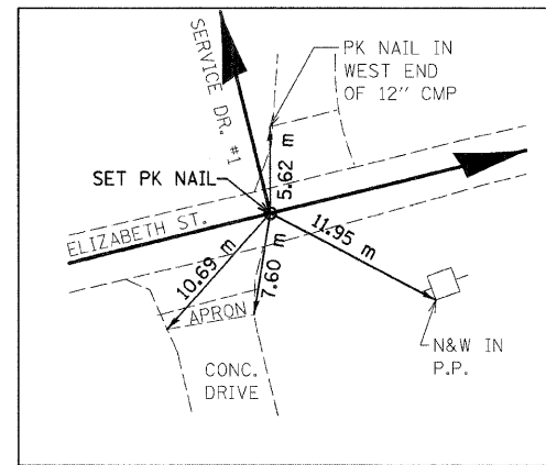
SERVICE DRIVE 1 POT STA 0+874.447 N 255,699.9455 E 698,357.3339
