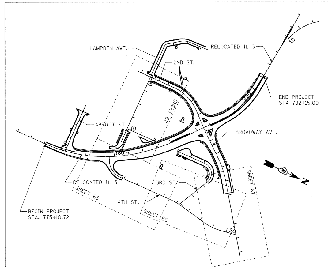
LOCAL ROAD RESURFACING SHEETS
