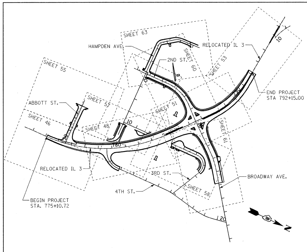
CONSTRUCTION PLAN SHEETS
