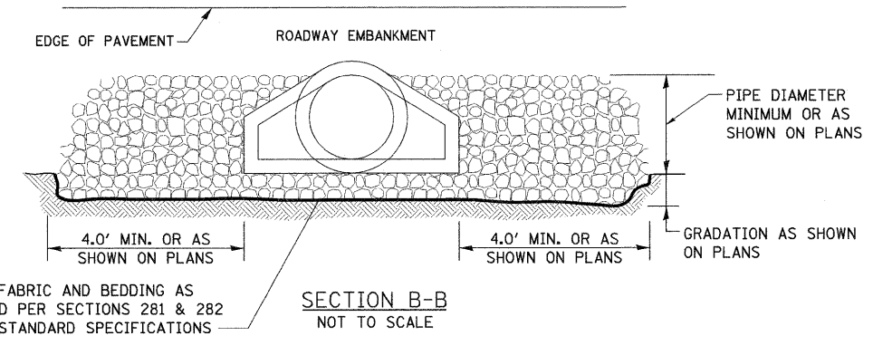
RIPRAP PROTECTION DETAIL IN DITCH NOT TO SCALE
