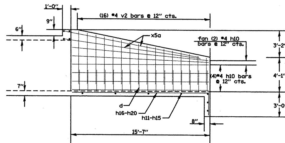
SECTION E-E LONG WINGWALL OUTSIDE WALL
