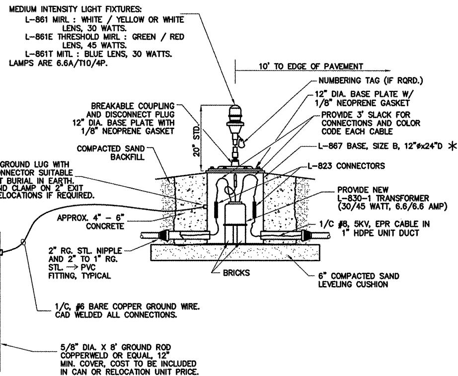
L-861 EDGE LIGHT INSTALLATION / RELOCATION DETAILS MEDIUM INTENSITY RUNWAY LIGHT (MIRL) MEDIUM INTENSITY TAXIWAY LIGHT (MITL) BASE MOUNTED, 6.6 AMP SERIES CIRCUIT NOT TO SCALE
