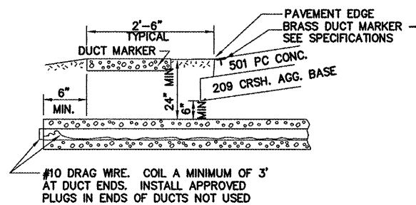
UNDERGROUND ELECTRICAL DUCT (NOT TO SCALE)
