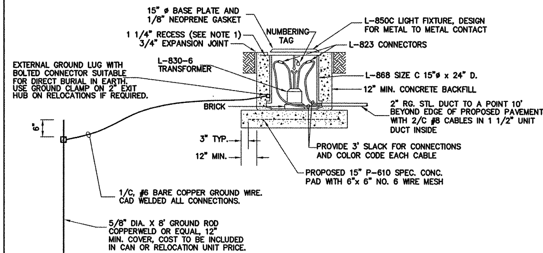
L-862 EDGE LIGHT INSTALLATION / RELOCATION DETAILS HIGH INTENSITY RUNWAY LIGHT / QUARTZ (HIRLQ) BASE MOUNTED, SERIES CIRCUIT NOT TO SCALE
