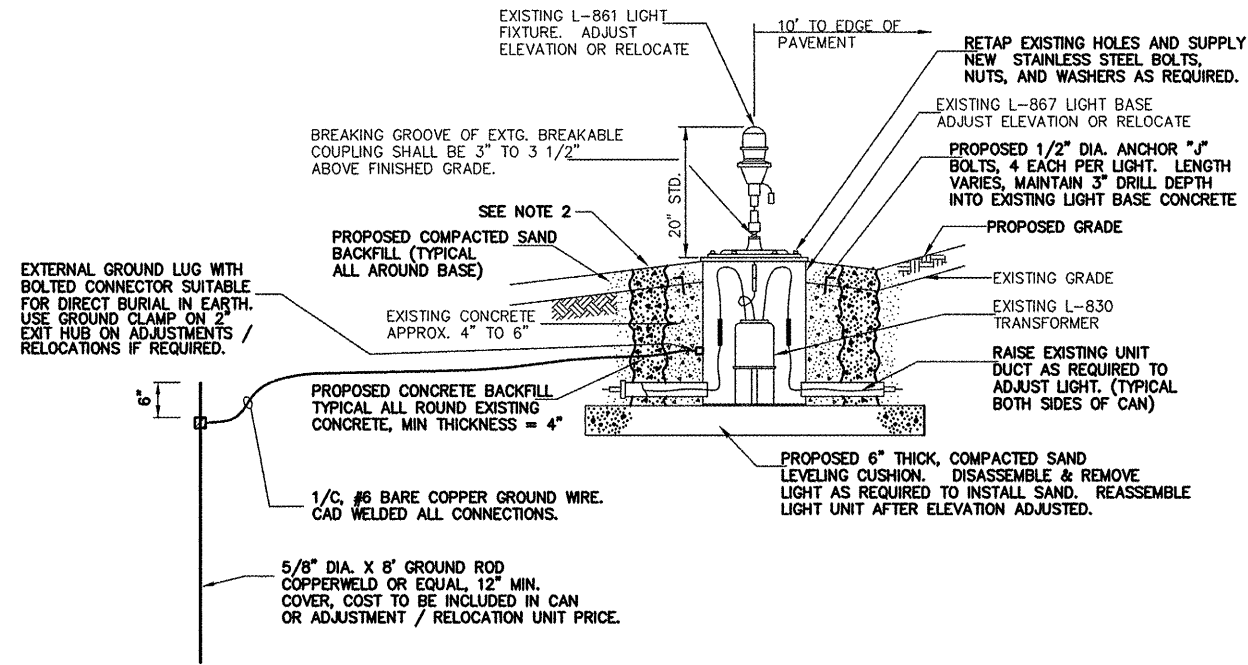
TYPICAL DETAIL L-861 EDGE LIGHTS ADJUSTMENT OR RELOCATION - IN TURF
