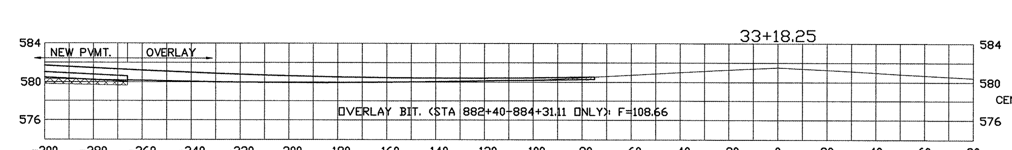
CENTERLINE PROFILE OF OLD TAXY E
