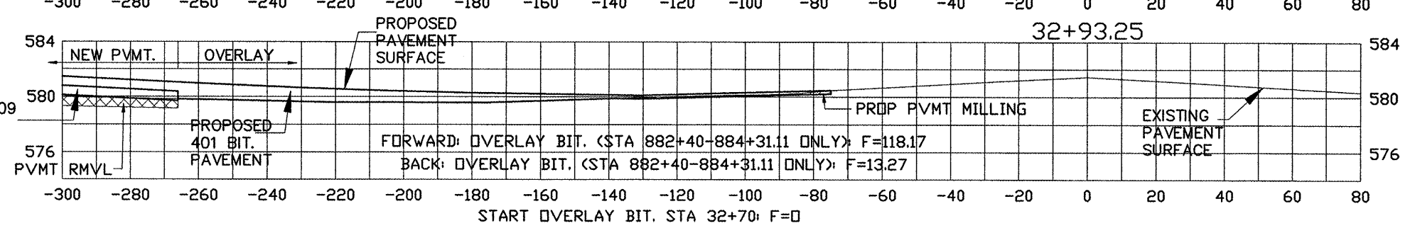
PROFILE OF SOUTH EDGE OF OLD TAXY E
