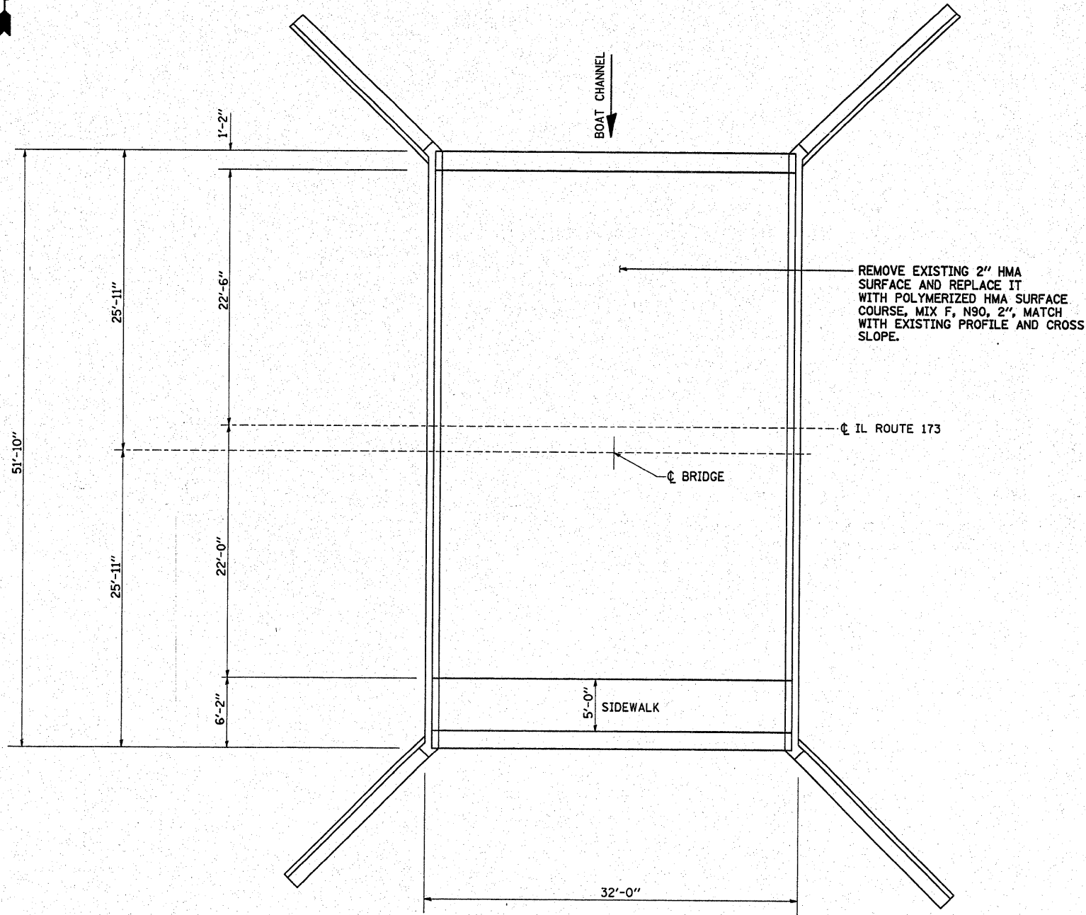
PLAN
