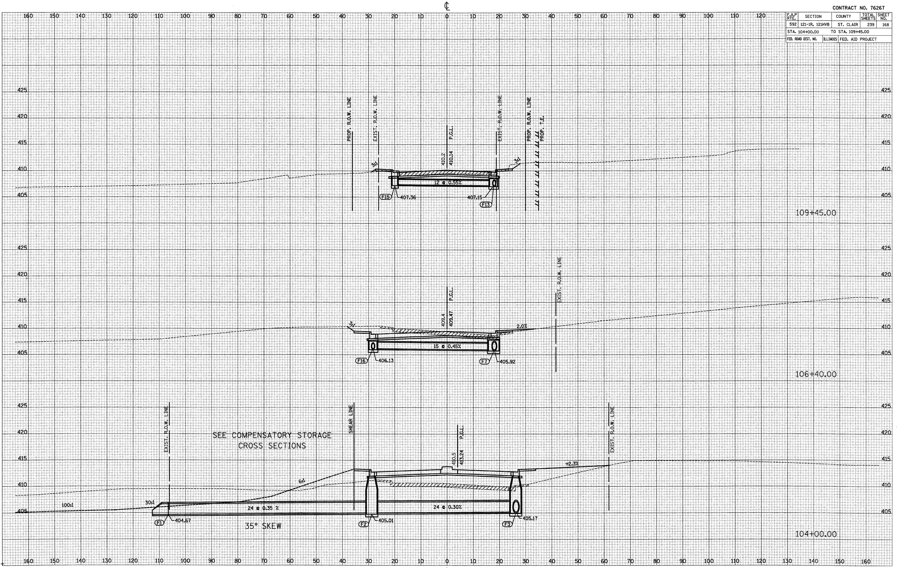
CULVERT PROFILES - RANGE LANE
