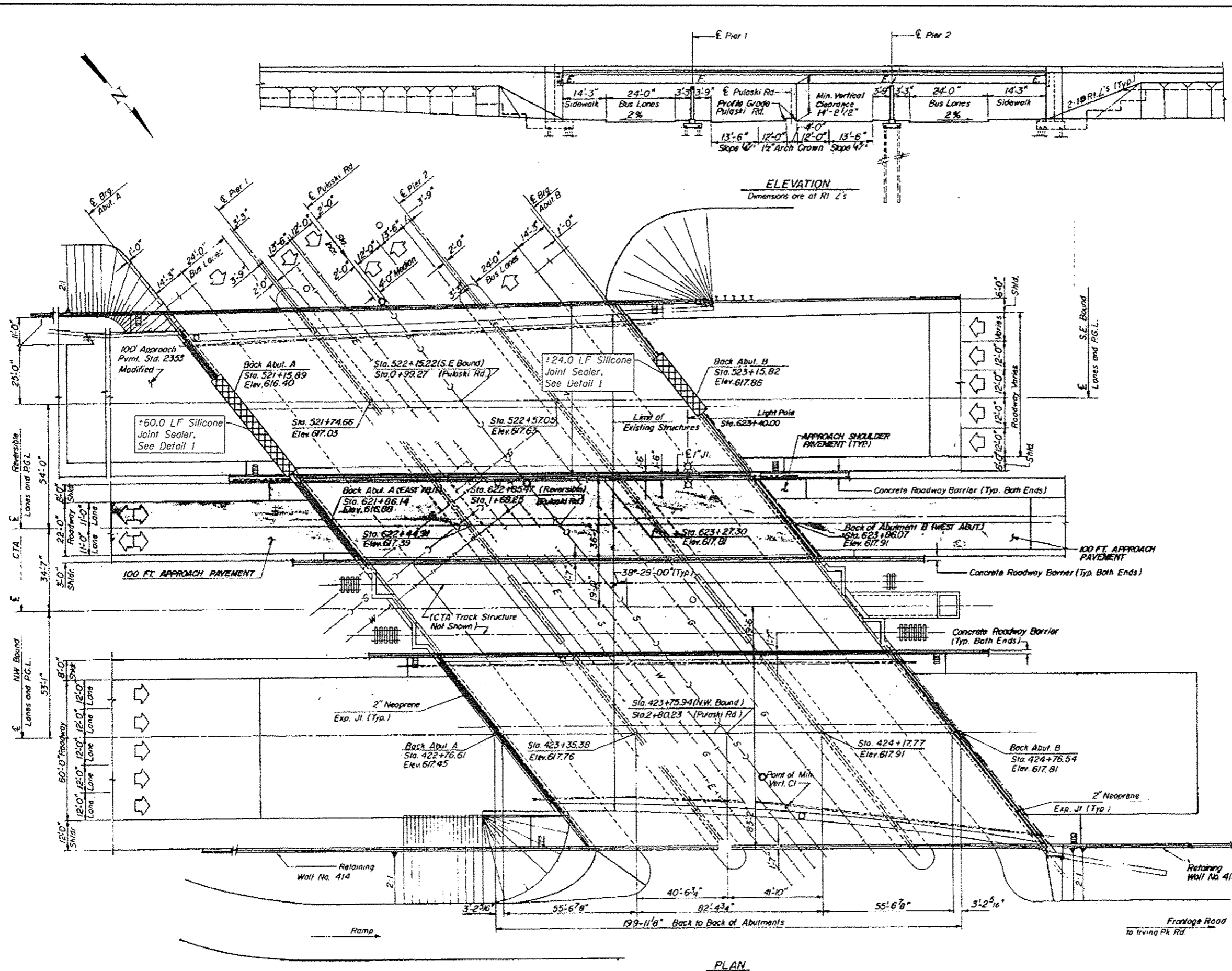
PLAN
