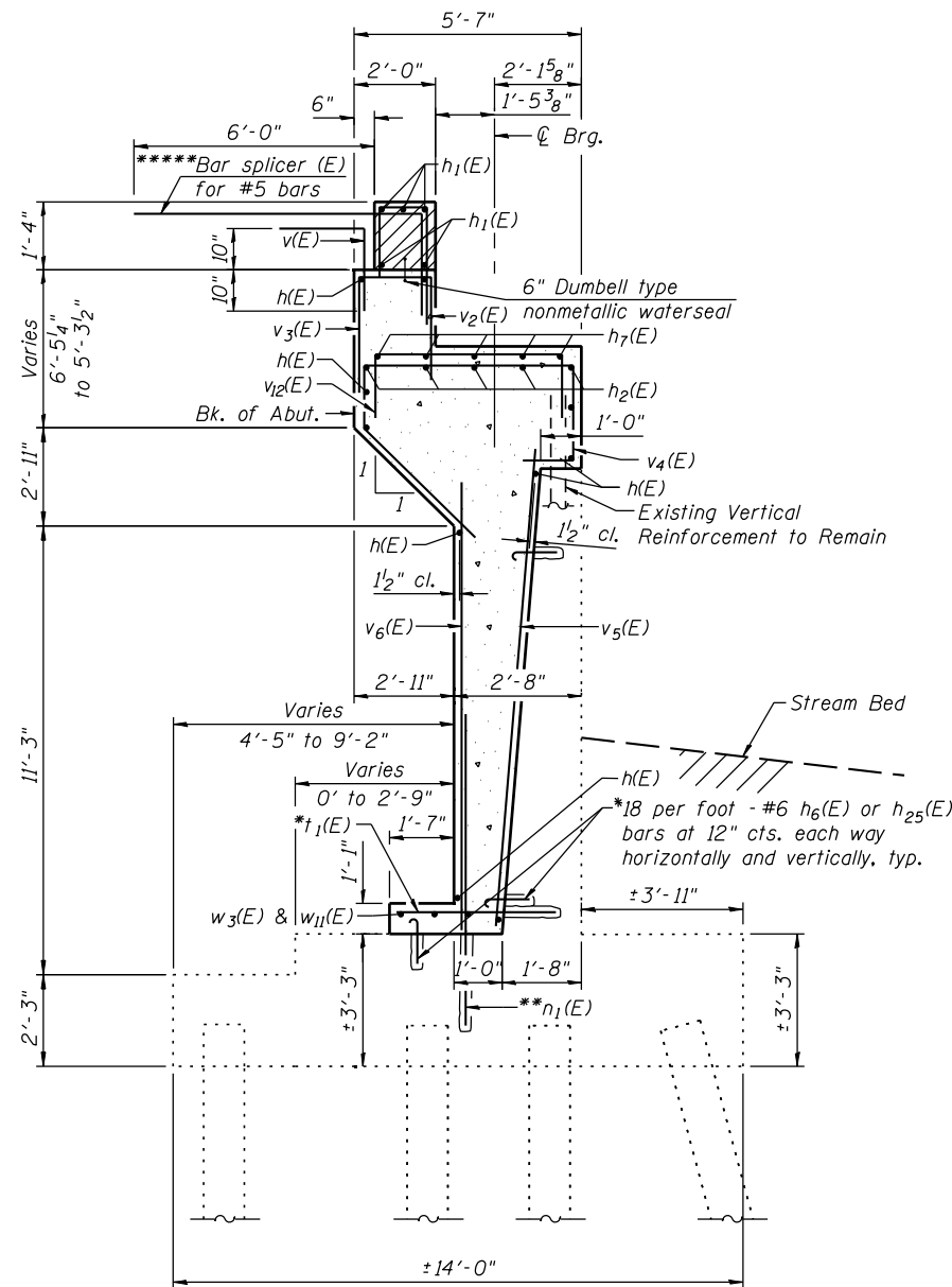
SECTION B-B
