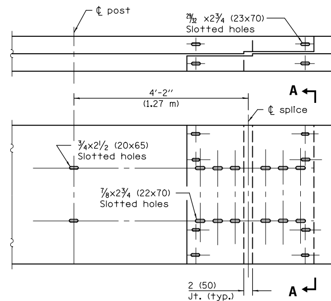
LAP SPLICE JOINT
