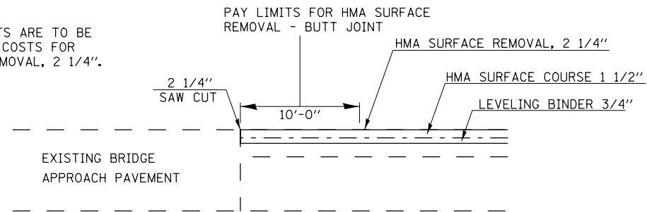
BUTT JOINT DETAIL #1
