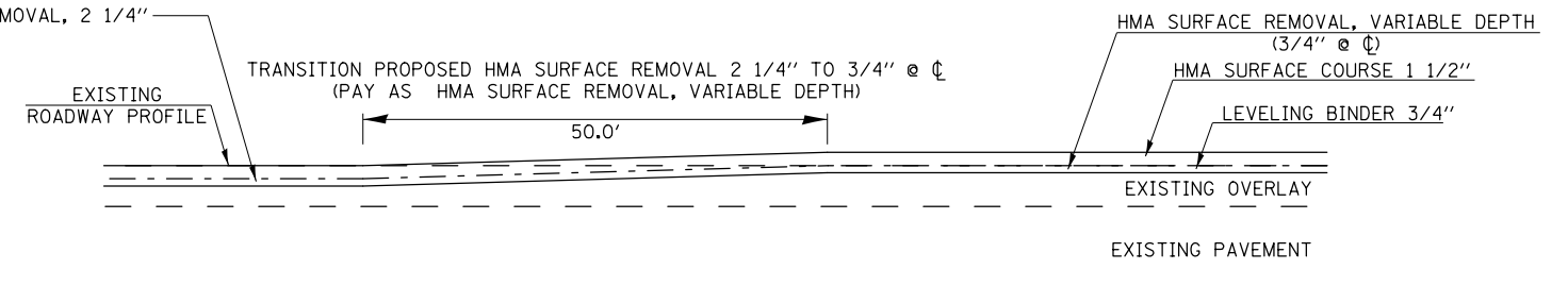
TRANSITION RAMP DETAIL #2
