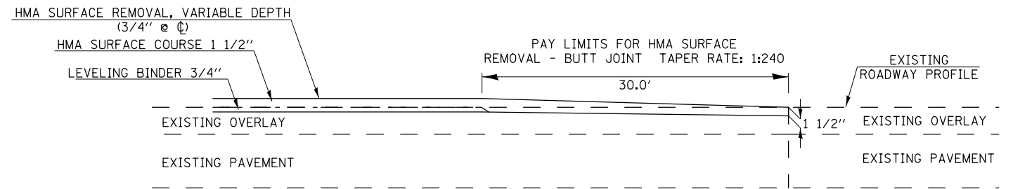
BUTT JOINT DETAIL #2
