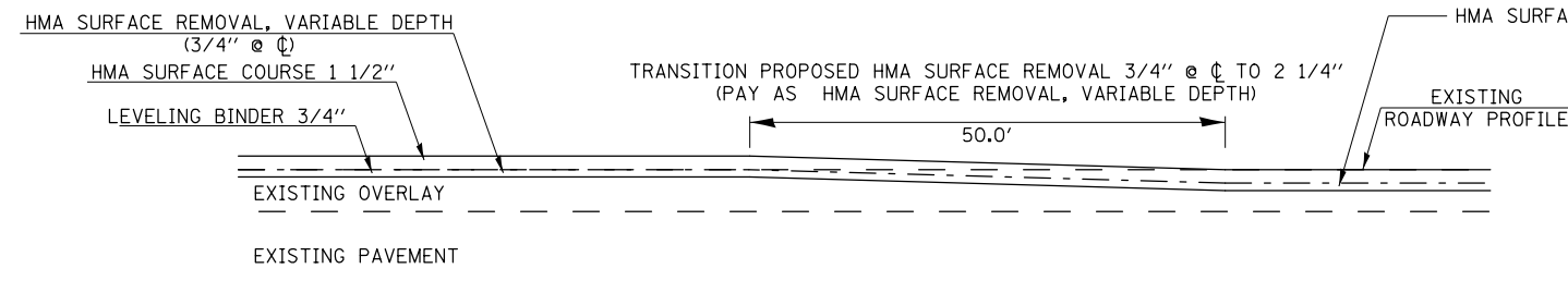
TRANSITION RAMP DETAIL #1
