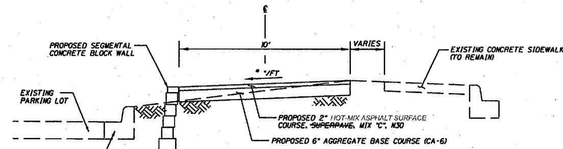
TYPICAL SECTION STA. 16+14.85 TO STA. 16+36.62 NOT TO SCALE
