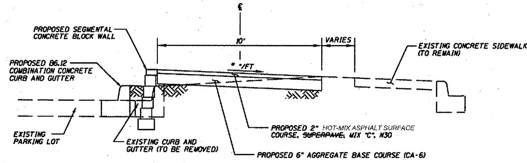
TYPICAL SECTION STA. 15+63.66 TO STA. 16+14.85 NOT TO SCALE
