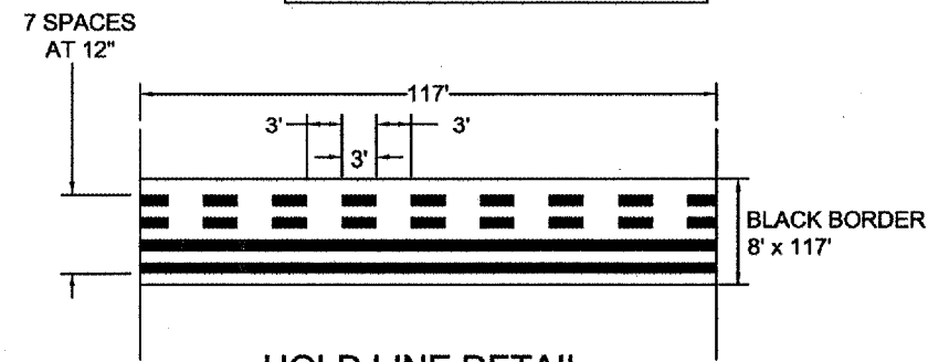
HOLD LINE DETAIL RUNWAY 6 TURNAROUND
