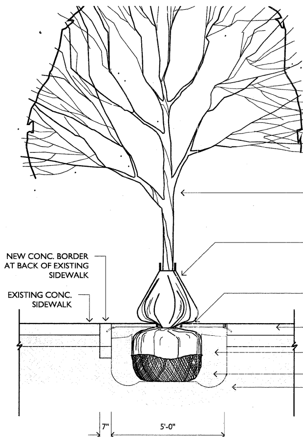
5 DECIDUOUS TREE IN TREE GRATE, SECTION PERPENDICULAR TO ROAD SCALE: 1/2" = 1'-0"
