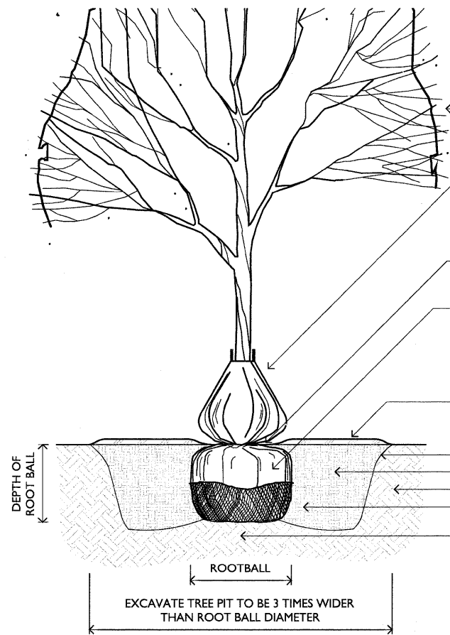
4 DECIDUOUS TREE IN TURF PARKWAY SCALE: 1/2" = 1'-0"
