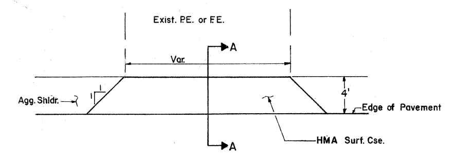
ENTRANCE DETAIL
