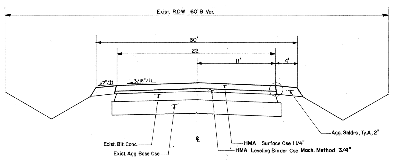
PROPOSED TYPICAL CROSS SECTION
