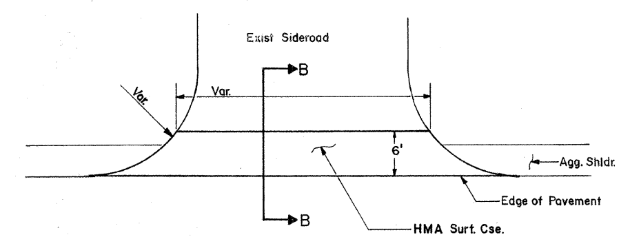
SIDEROAD DETAIL
