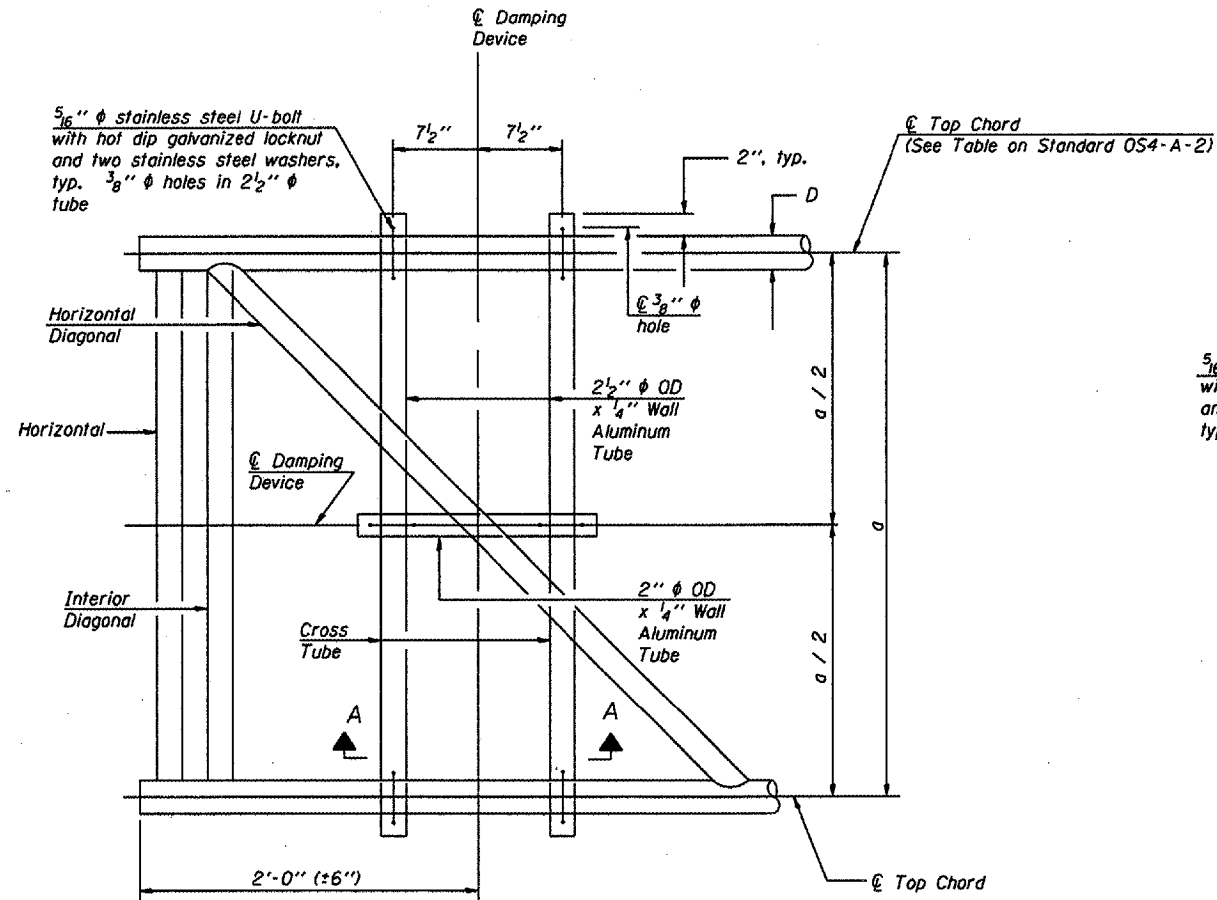
PLAN DETAIL
