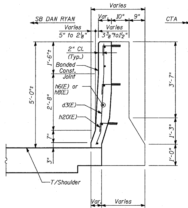
SECTION F-F
