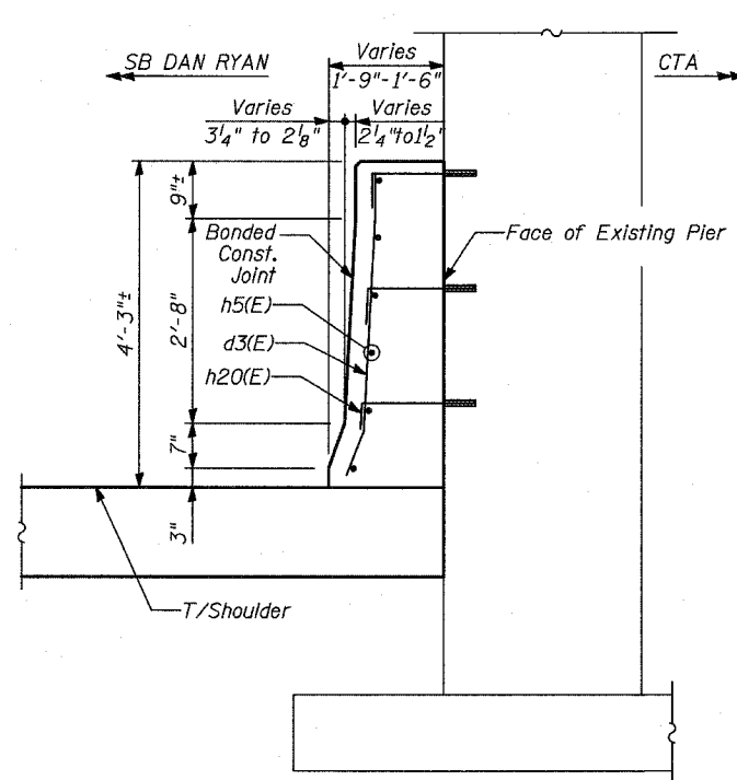
SECTION C-C
