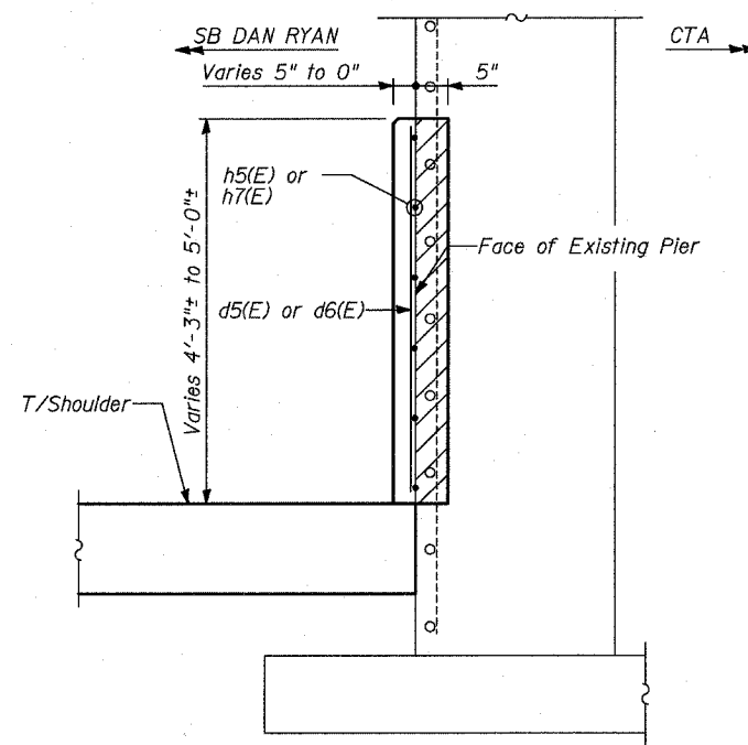
SECTION E-E
