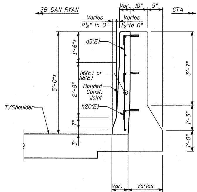
SECTION G-G
