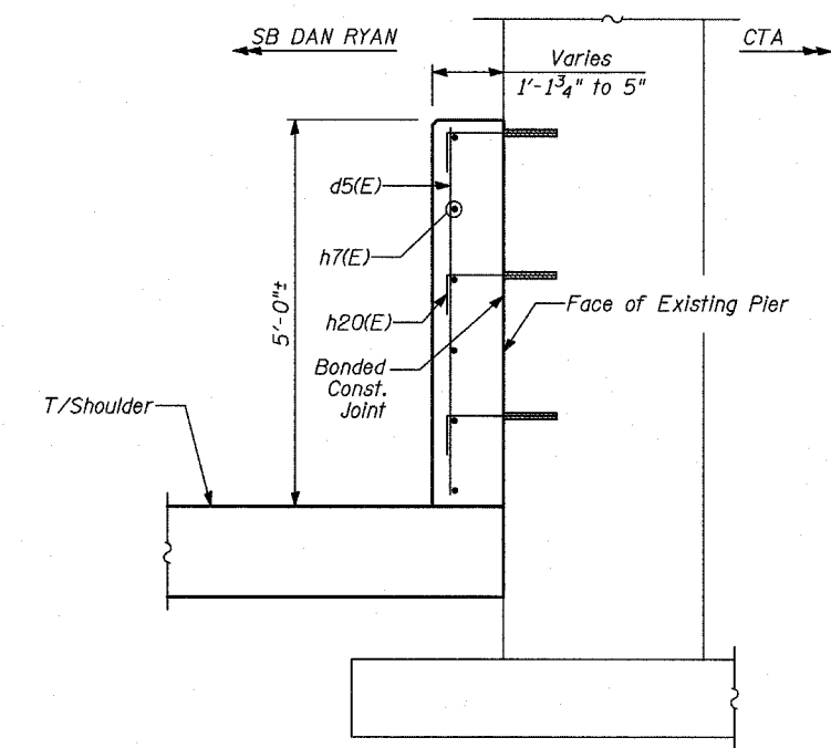
SECTION H-H
