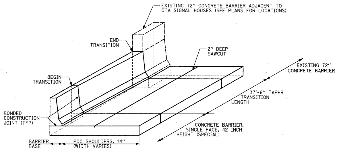
72" CONCRETE BARRIER TRANSITION DETAIL NO SCALE
