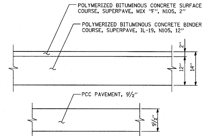
TEMPORARY PAVEMENT DETAILS (CONTRACTOR HAS THE OPTION OF USING BITUMINOUS OR PCC SECTION FOR TEMPORARY PAVEMENT) SCALE: 1"=1'-0"
