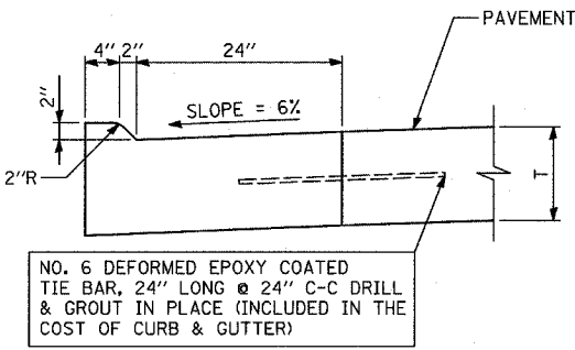
COMBINATION CONCRETE CURB & GUTTER, TYPE M-2.24 SCALE: 1"=1'-0"
