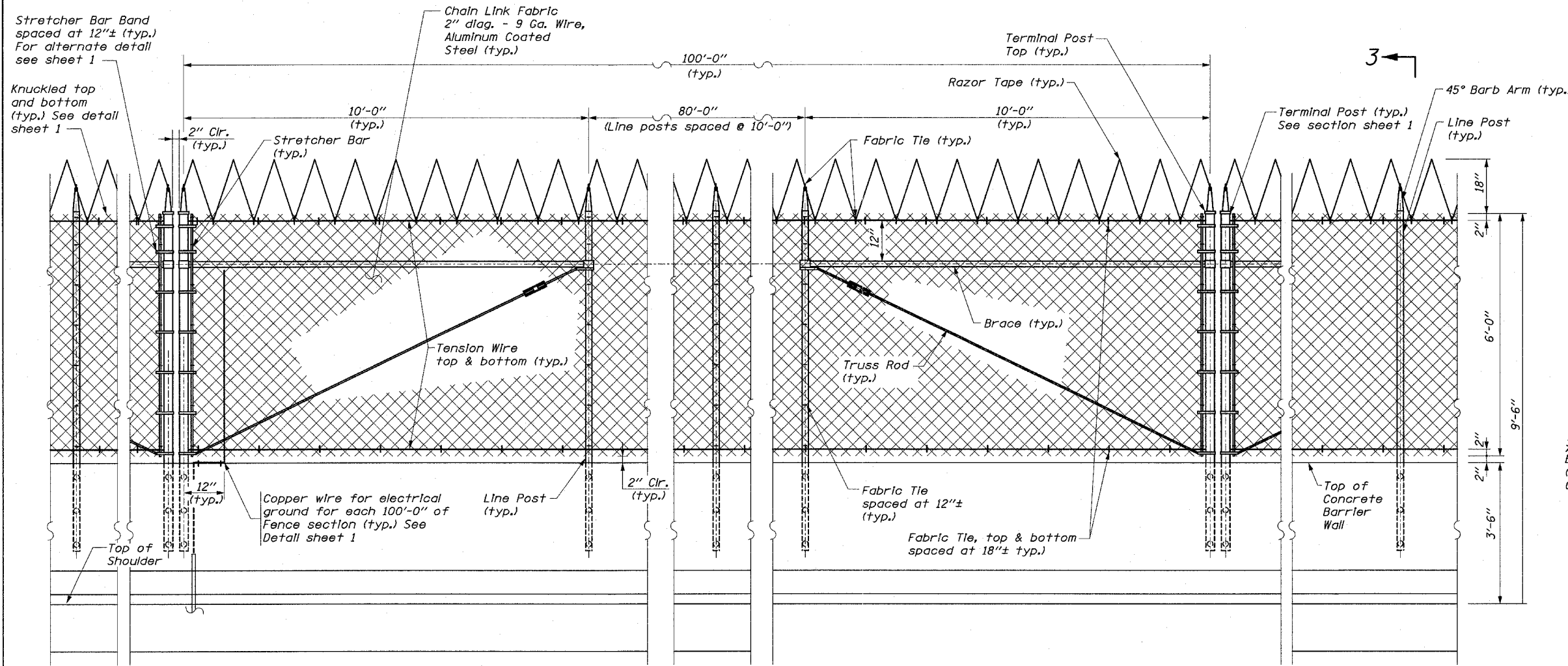
ELEVATION CTA FENCE (SPECIAL) ON CONCRETE BARRIER WALL
