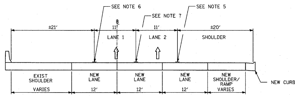
JJ-JJ STAGE 3D: SB I-57; STA. 87+48 TO 97+48
