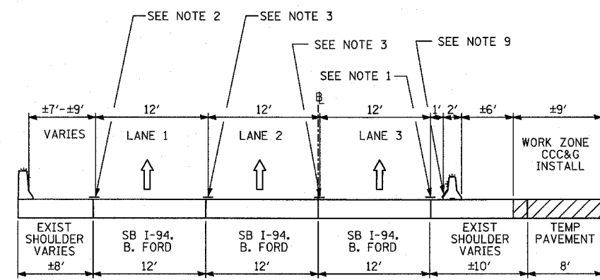
FF-FF STAGE 3C: SB I-94 BISHOP FORD; STA. 1127+00 TO STA. 1143+04
