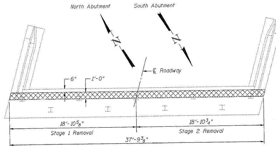
ABUTMENT PLAN
