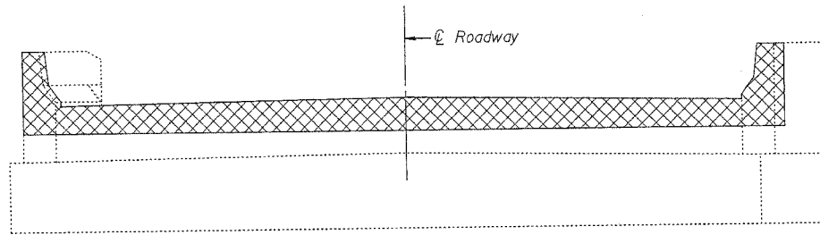
ABUTMENT ELEVATION
