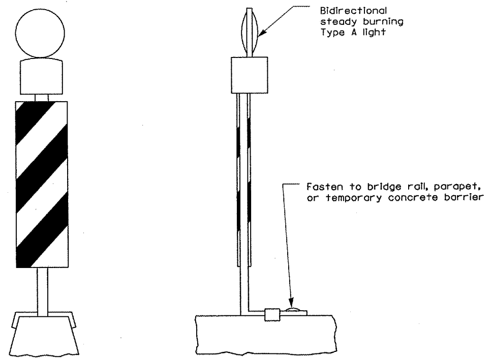
(Suggested mounting detail)
