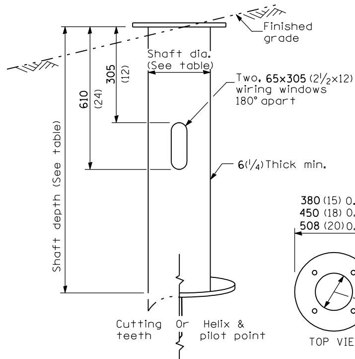
STEEL FOUNDATION
