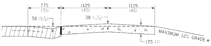
DESCENDING APPROACH
