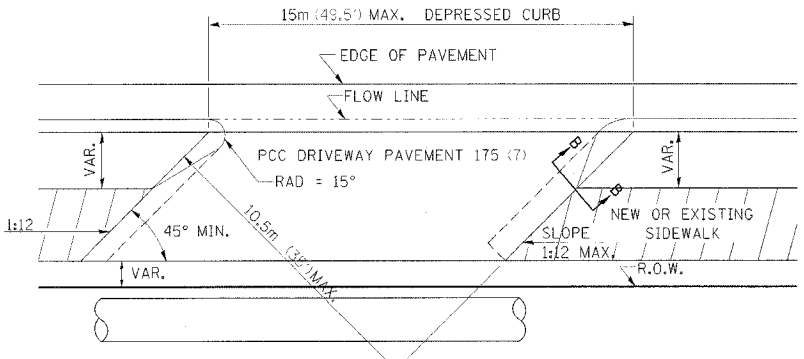
COMMERCIAL ENTRANCE
