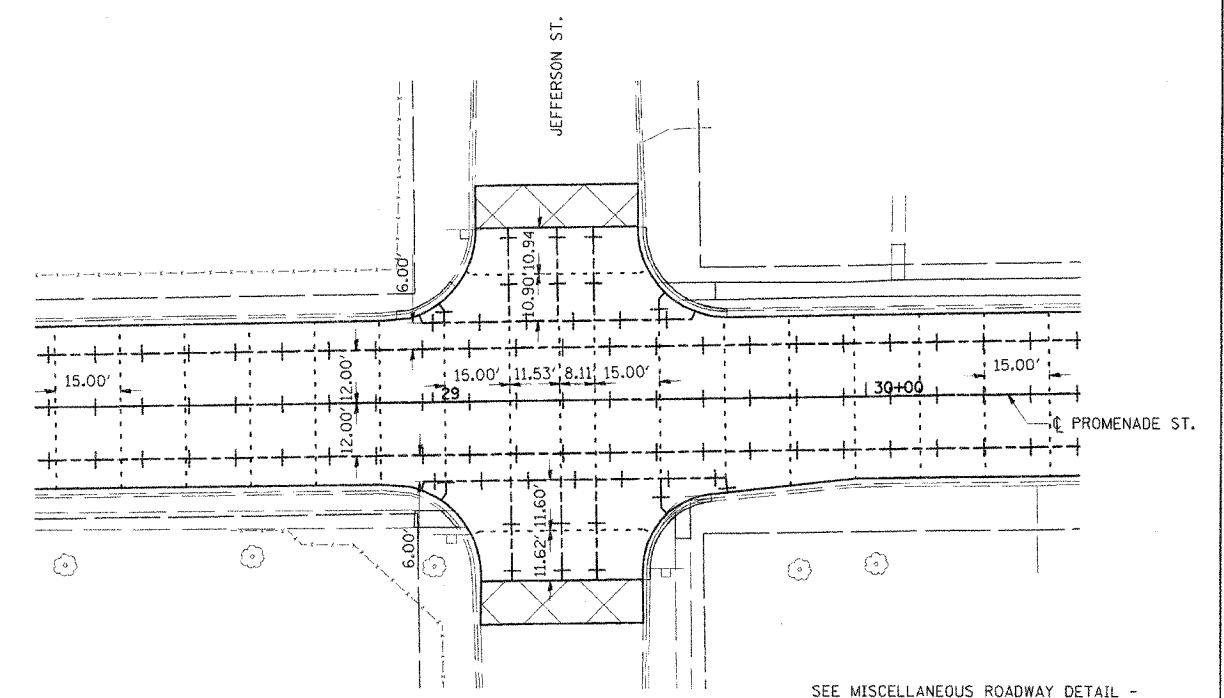
JOINTING PLAN
