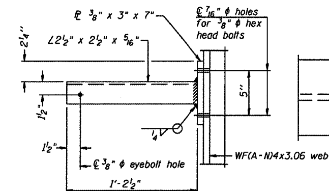
SECTION P-P
