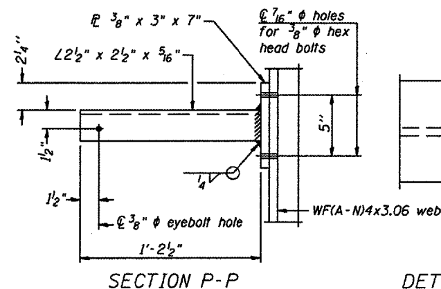
ALTERNATE SAFETY CHAIN ATTACHMENT
