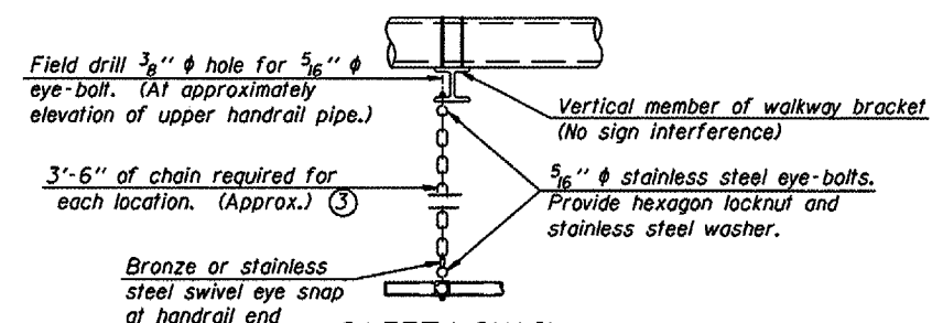
SAFETY CHAIN
