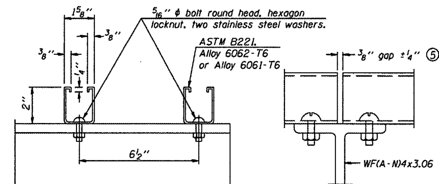
SECTION F-F
