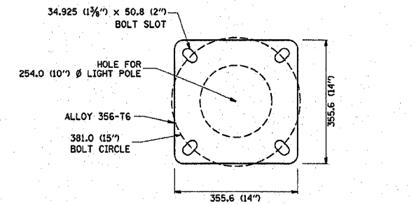
LIGHT POLE BASE PLATE DETAIL (FOR POLE MOUNTED ON 381.0 (15 INCH) BOLT CIRCLE FOUNDATION)
