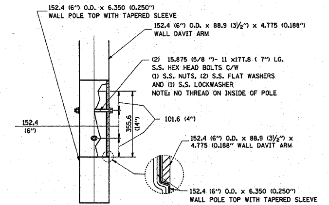
DAVIT ARM CONNECTION [355.6 (14") OVERLAP SHOWN]
