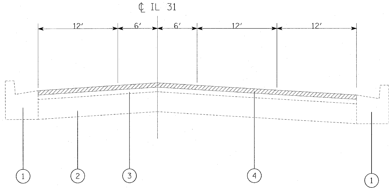
EXISTING TYPICAL CROSS SECTION IL 31 (RICHMOND ROAD) STA. 2+75 TO 5+56
