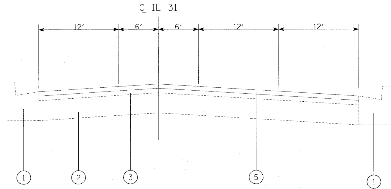
PROPOSED TYPICAL CROSS SECTION IL 31 (RICHMOND ROAD) STA. 2+75 TO 5+56
