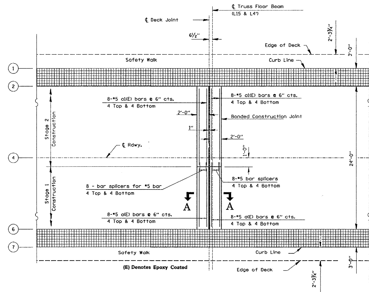
PROPOSED DECK PLAN Truss Spans @ L15 & L4'
