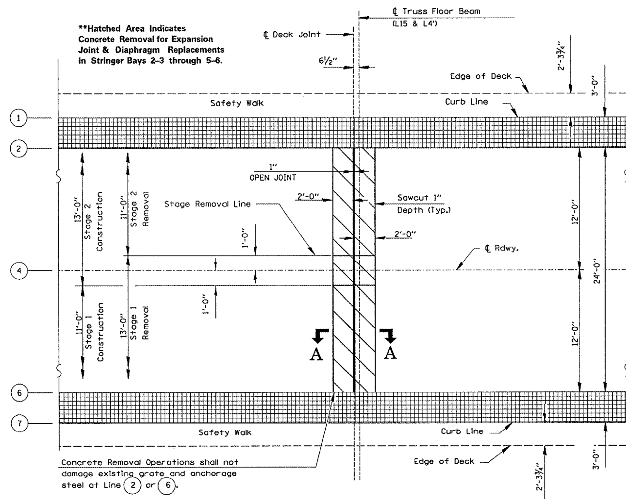
EXISTING DECK PLAN Truss Spans @ L15 & L4'
