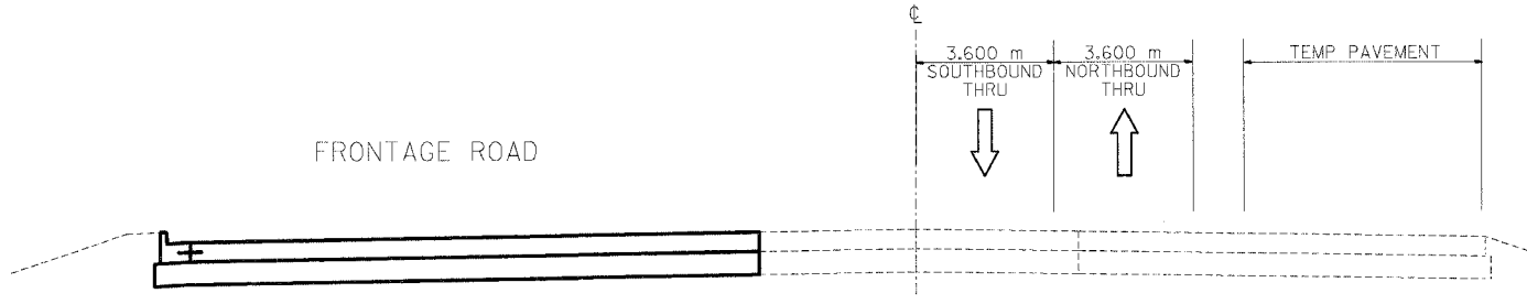
ALTORFER LANE MOT TYPICAL SECTION STEP F ALTORFER LANE @ NORTH MAIN ST.
