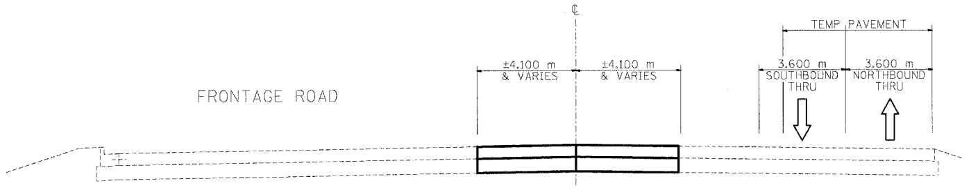
ALTORFER LANE MOT TYPICAL SECTION STEP E ALTORFER LANE @ NORTH MAIN ST.
