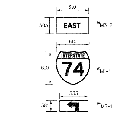
10 TEMPORARY SIGN PANEL ASSEMBLY MAIN ST. STAGE 3A-1 (PRE-STAGE 3) STA. 2+520
