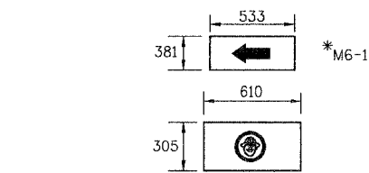
6 TEMPORARY SIGN PANEL ASSEMBLY CAMP ST. (STAGE 3A) STA. 2+571
