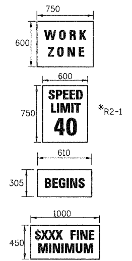
9 TEMPORARY SIGN PANEL ASSEMBLY MAIN ST. (STAGE 3A) STA. 2+175 MAIN ST. STAGE 3A-1 (PRE-STAGE 3) STA. 4+278
