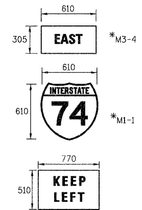
14 TEMPORARY SIGN PANEL ASSEMBLY MAIN ST. (STAGE 3A-3) STA. 2+605
