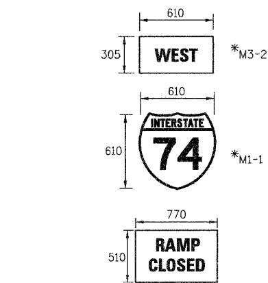
13 TEMPORARY SIGN PANEL ASSEMBLY MAIN ST. (STAGE 3A-3) STA. 2+605
