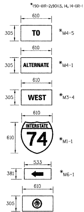
6 TEMPORARY SIGN PANEL ASSEMBLY CAMP ST. (STAGE 3A) STA. 2+571
