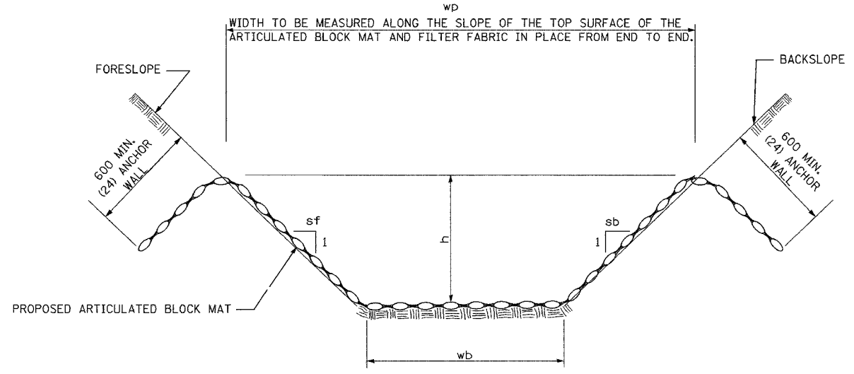
TYPICAL ARTICULATED BLOCK MAT LINED DITCH
