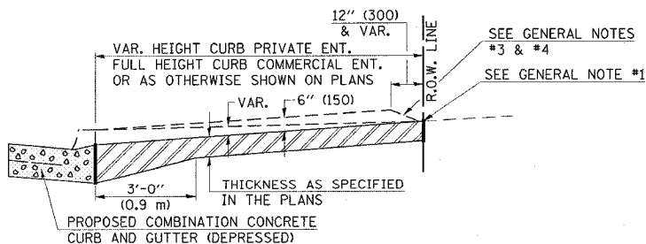
SECTION A-A WITHOUT SIDEWALK
