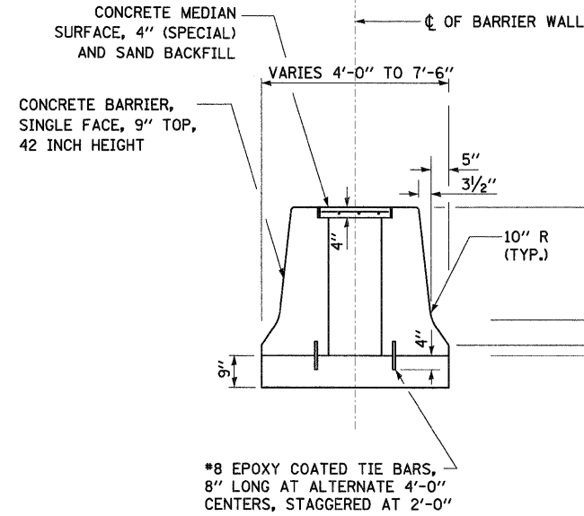
SECTION C-C
