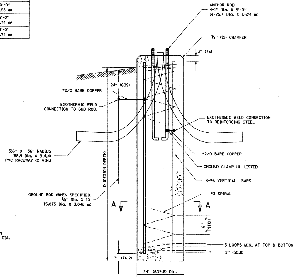
FOUNDATION DETAIL
