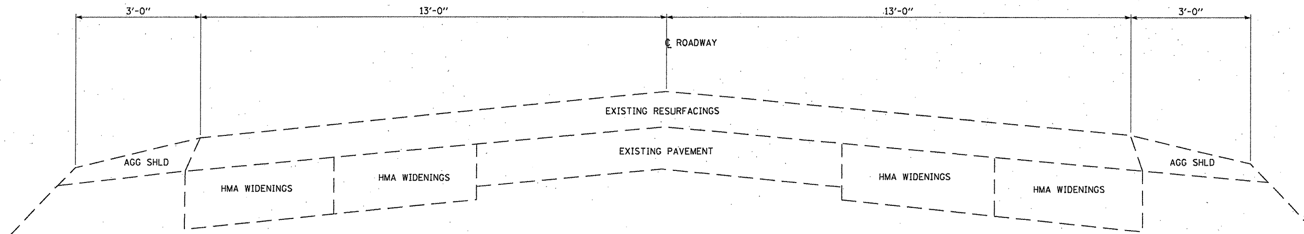
TYPICAL SECTION
