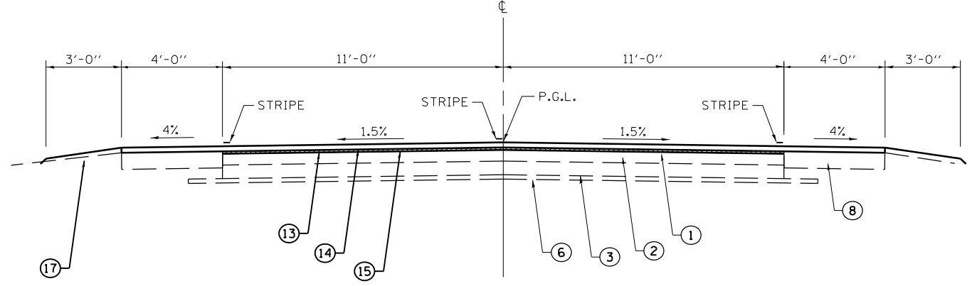
TYPICAL CROSS SECTION - IL. RTE. 29
