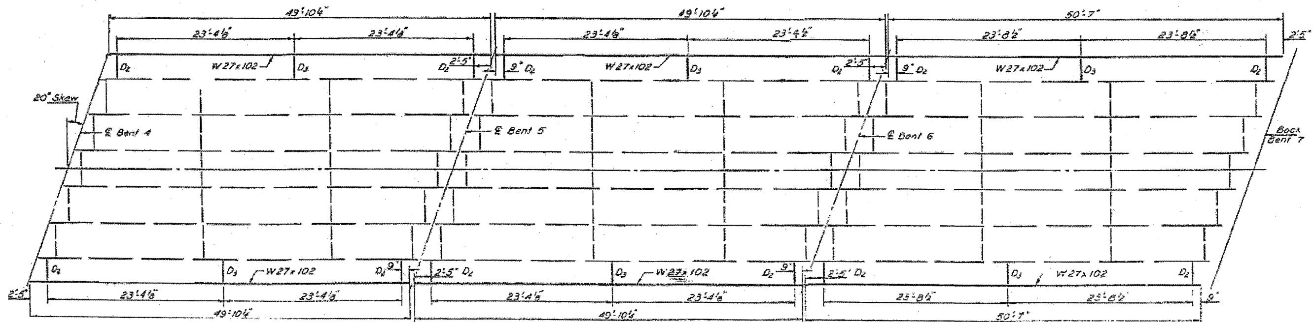
FRAMING PLAN
