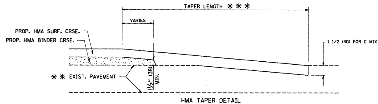
HMA TAPER DETAIL
