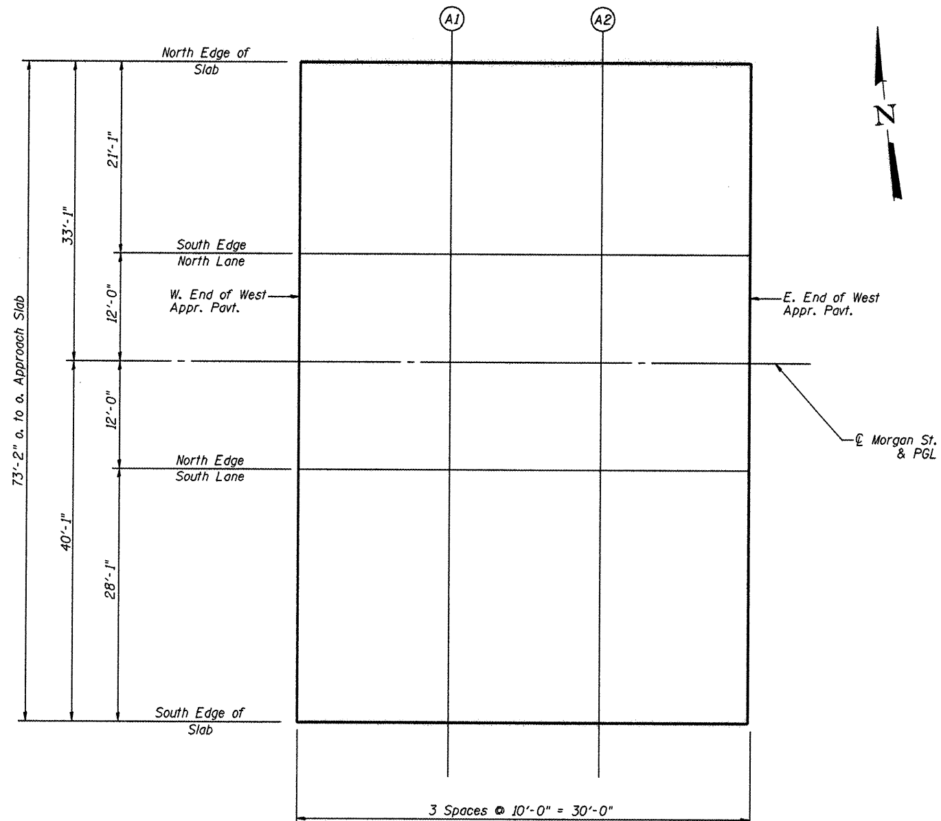
PLAN - WEST APPROACH
