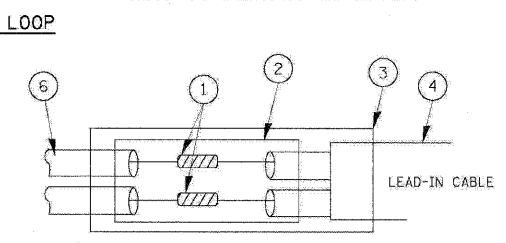
DETAIL "B" LOOP-TO-CONTROLLER SPLICE
