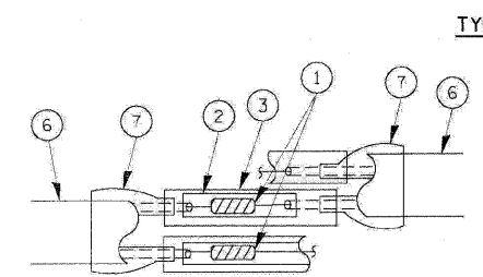
DETAIL "A" LOOP-TO-LOOP SPLICE
