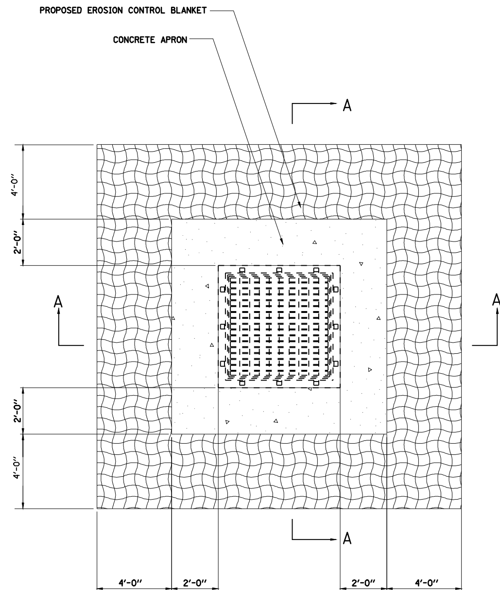
PLAN VIEW
