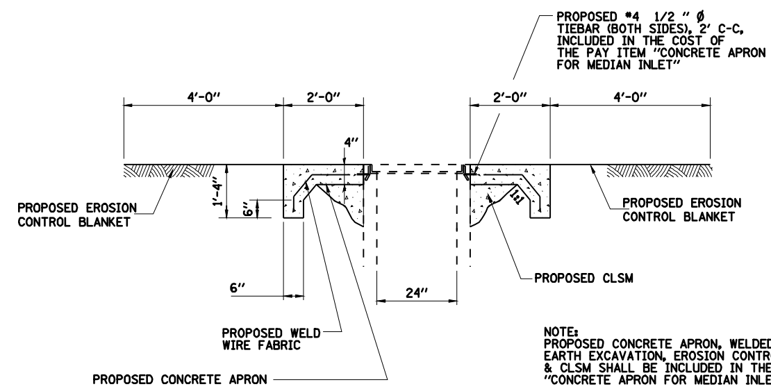
SECTION A-A CONCRETE APRON FOR MEDIAN INLET BOX (542546)
