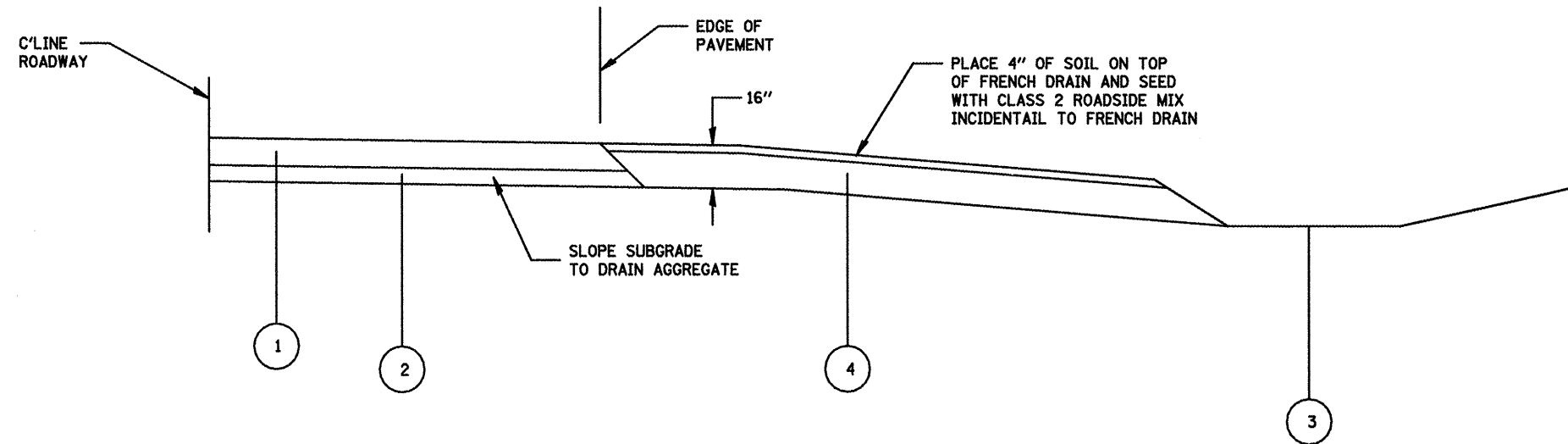
STANDARD DETAIL OF FRENCH DRAIN AT CLASS C PATCHES
