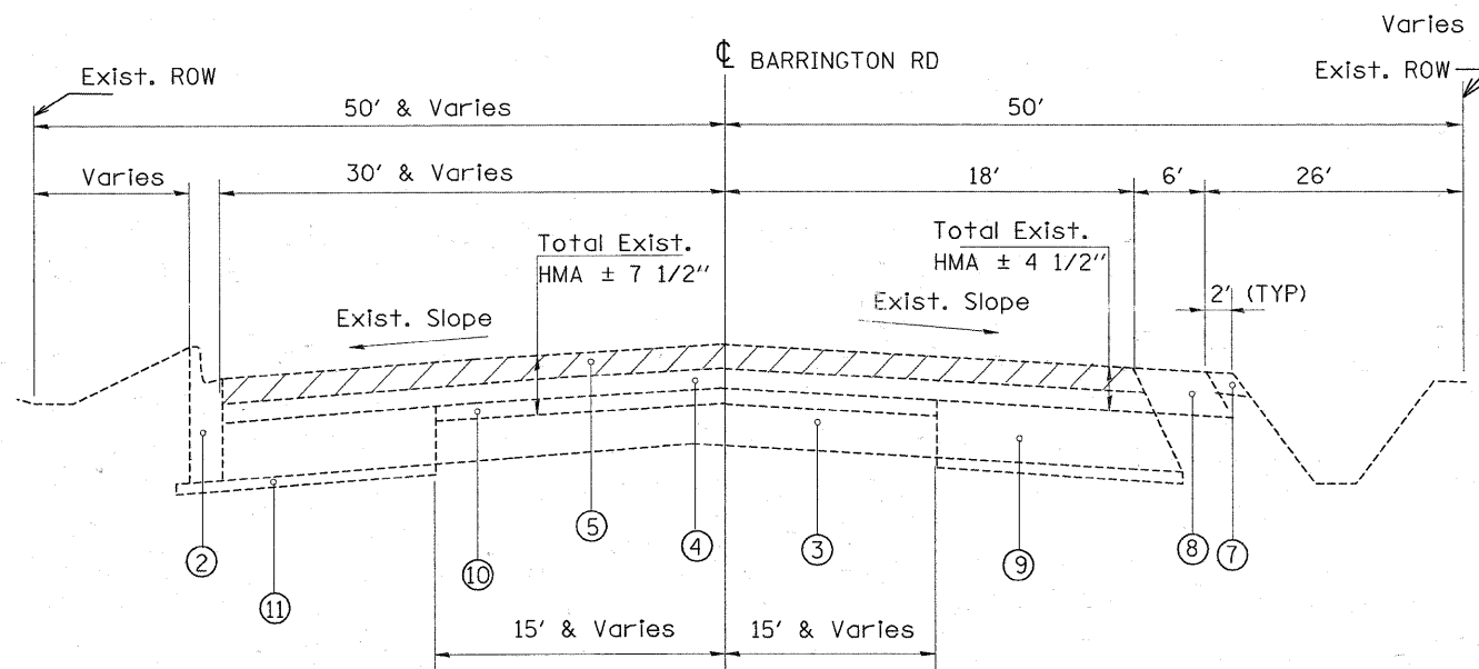
EXISTING TYPICAL SECTION STA 75+41.38 TO STA 78+58.6
