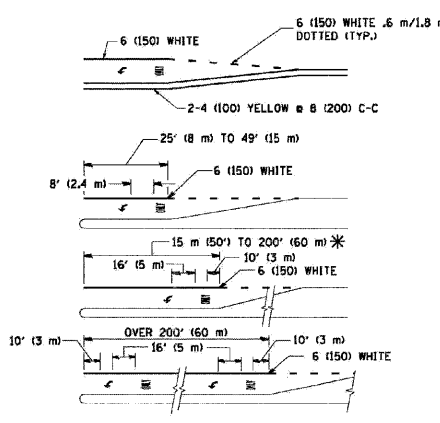
TYPICAL PAINTED MEDIAN MARKING
