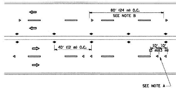
MULTI-LANE/UNDIVIDED
