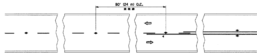
TWO-LANE/TWO-WAY
