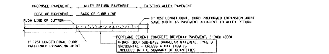
ALLEY RETURN DETAIL
