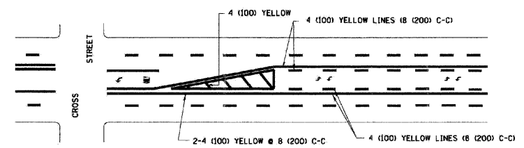
PAINTED MEDIANS
