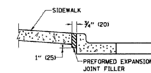
SLOPE FOR SIDEWALK 1" (25) IN 3'-0" (0.9 m) IN CHICAGO
