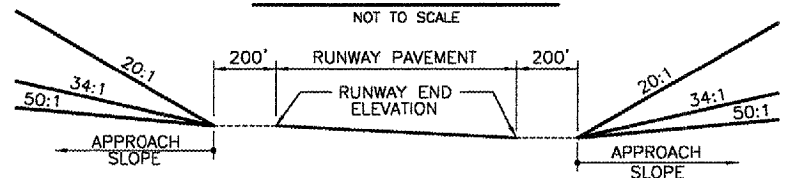
TYPICAL PROFILE F.A.R. PART 77 IMAGINARY SURFACES
